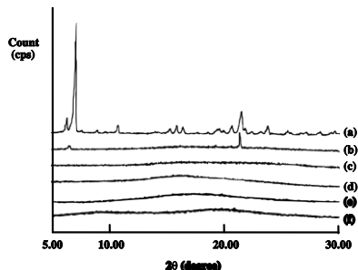
Fig. 1. Powder X-ray diffraction (PXRD) patterns of (a) FP crystal, (b) PM of FP/Hsp-G (1/10), (c) SPD of FP/Hsp-G (1/10), (d) SPD of FP/Stevia-G (1/10), (e) SPD of FP/HPMC (1/10), (f) Hsp-G powder.
