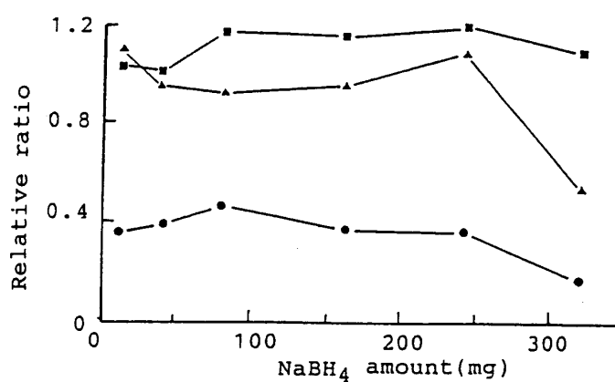
Fig.3 : Effect of NaBH 4 Amount (●) : methyltin chloride, (▲) : dimethyltin dichloride, (■) : trimethyltin chloride
